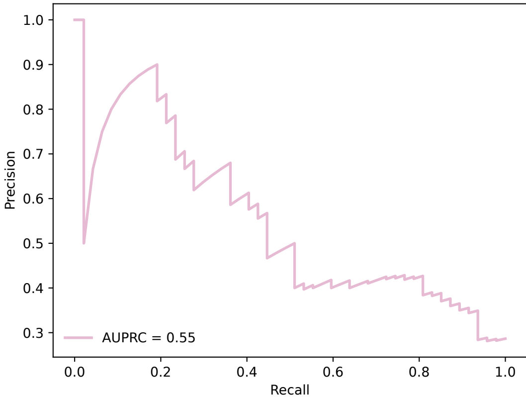
MLP Precision-Recall Curve
